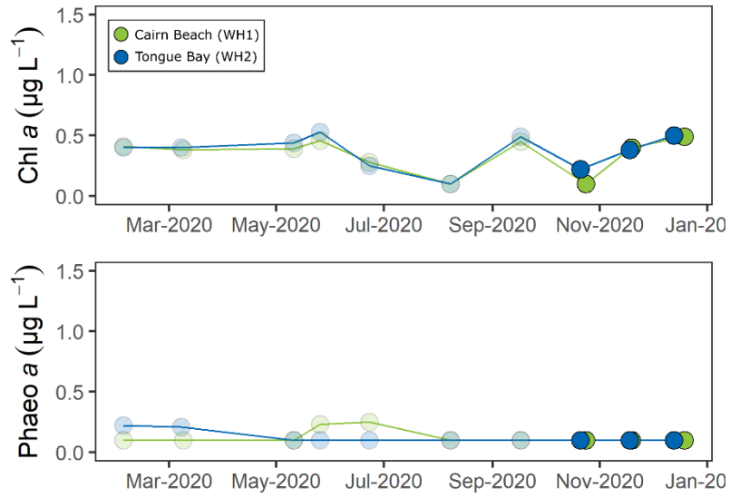
Figure 11. Chlorophyll a and phaeophytin a concentrations measured in water samples collected from Cairn Beach WH1 (green) and Tongue Bay WH2 (blue) 2020.
